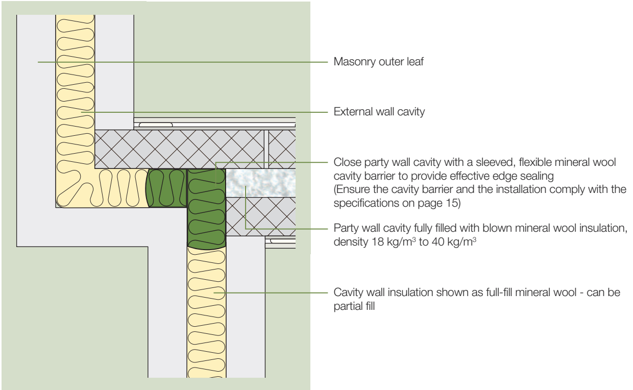
Figure MD3 Staggered External (Flanking) Wall Junction
