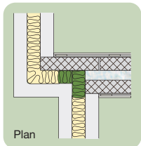
Figure MD3 Staggered wall junction See p.12 For equivalent timber detail Figure TD3 see p.18
