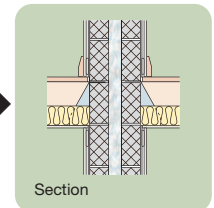
Figure MD4a Internal floor junction See p.12
