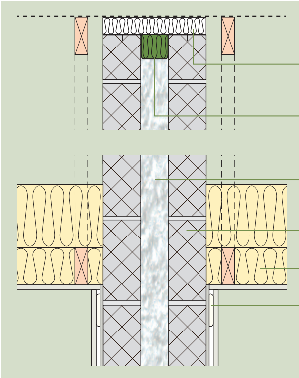
Figure MD7 Roof Junction – Pitched Roof Without Room-In-Roof
